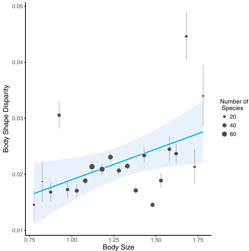
Figure 4. Relationship between body shape disparity, measured as Procrustes variance, and body size, measured as log-centroid size ( R^2 = 0.237 , P = 0.019 ). Point size corresponds to the number of species in a given body size interval. The shaded region is the 95% confidence interval around the regression line.
