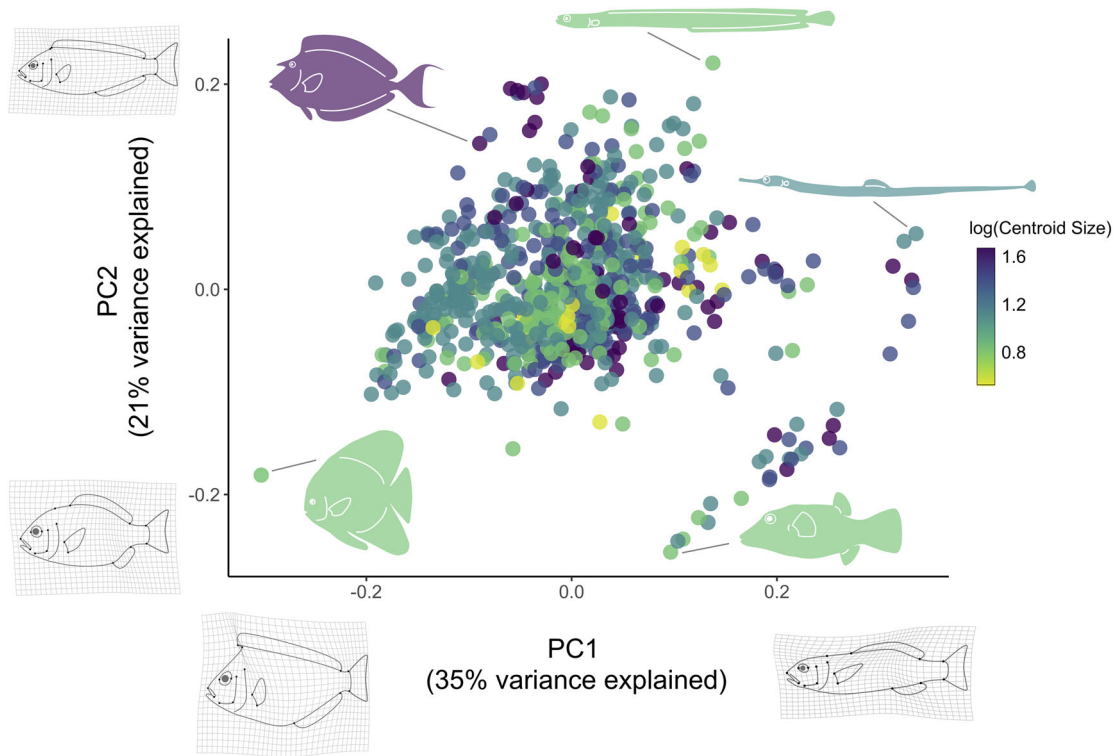
Figure 2. Plot of principal components 1 and 2, together accounting for 56.5% of total body shape variation across the dataset. Principal component analysis was conducted on the shape coordinates from 17 landmarks across 791 species. Point color corresponds to the log of centroid size in each species. Body shape variation along both PC 1 and 2 is shown as warp grids along the axes. Shapes of five species distributed across the morphospace are illustrated, clockwise from the upper left: Naso unicornis , Gunnelichthys pleurotaenia , Corythoichthys intestinalis , Canthigaster janthinoptera , and Platax teira .
